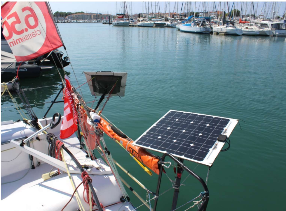
2x holder of the solar modul
